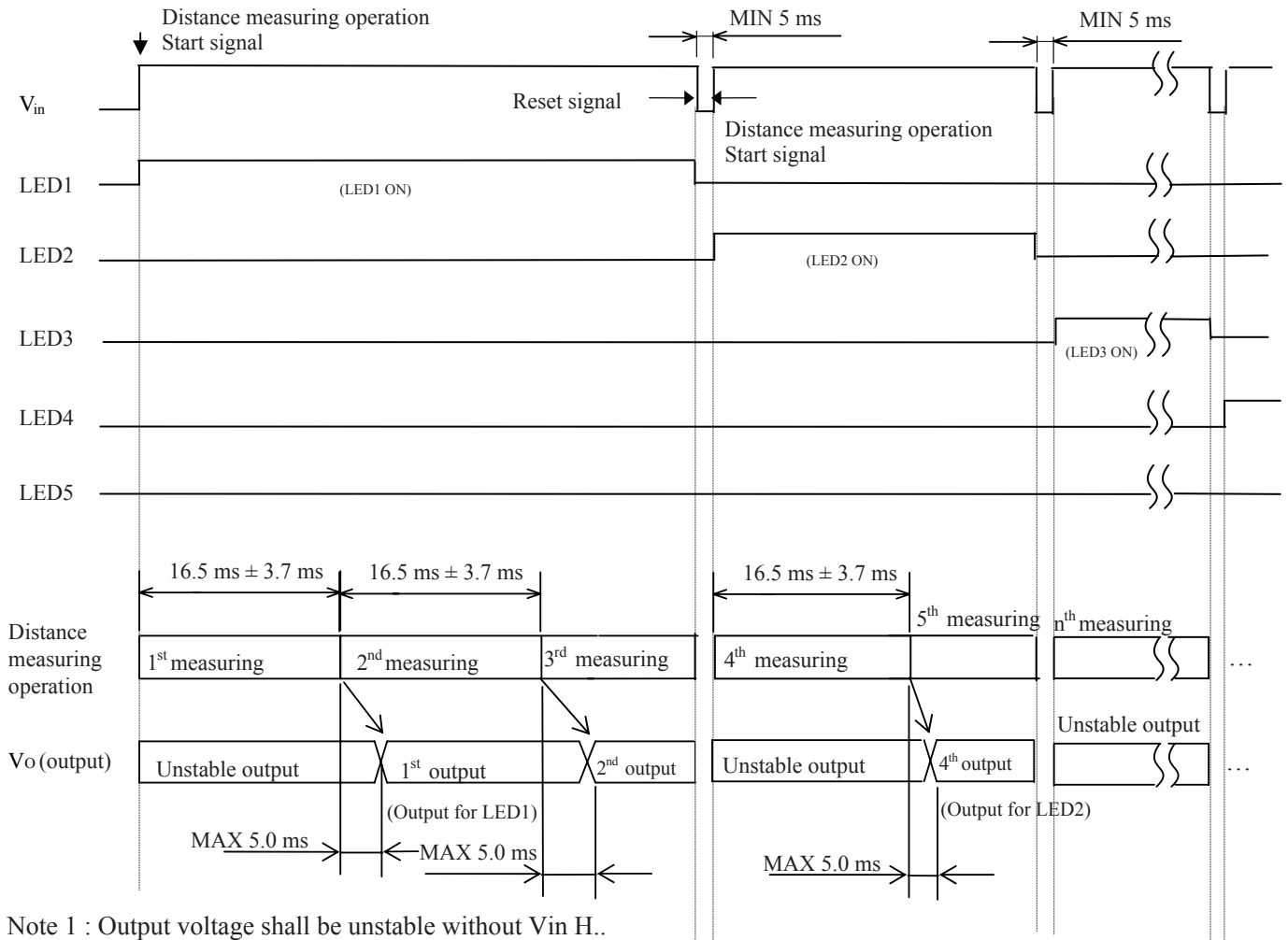
Fig. 1 Timing chart
